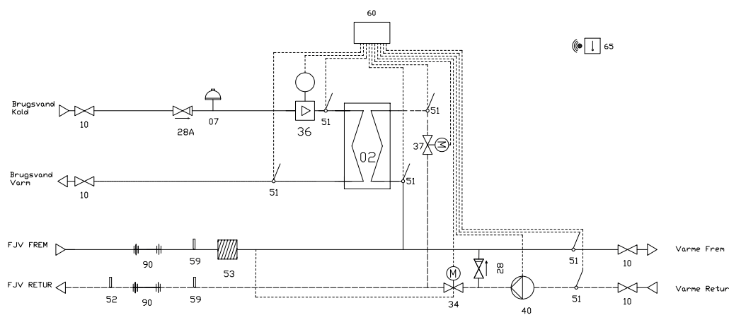
Principdiagram, Calefa II S ITC
