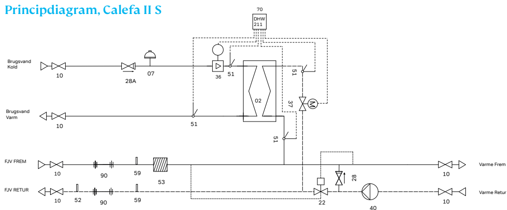
Principdiagram, Calefa II S ITC
